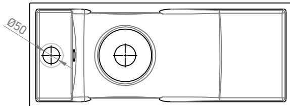
Bottom view
